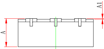
SIDE VIEW [侧视图]
